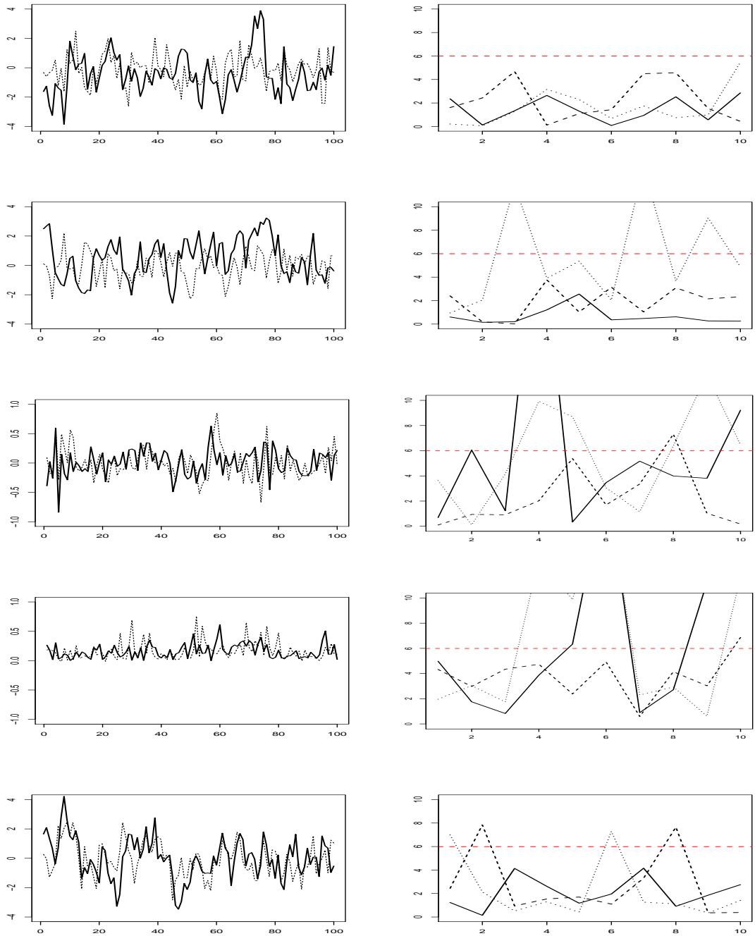
Figure 1: Stationary case: Bivariate realizations (left panels) and DFT covariances (right panels) T|\widehat{C}_{11}(r,0)|^2 (solid), T|\sqrt{2}\widehat{C}_{21}(r,0)|^2 (dashed) and T|\widehat{C}_{22}(r,0)|^2 (dotted) for stationary models S(I)–S(V) (top to bottom). The dashed red line is the 0.95-quantile of the \chi^2 distribution with two degrees of freedom and DFT covariances are reported for sample size T = 500 .
